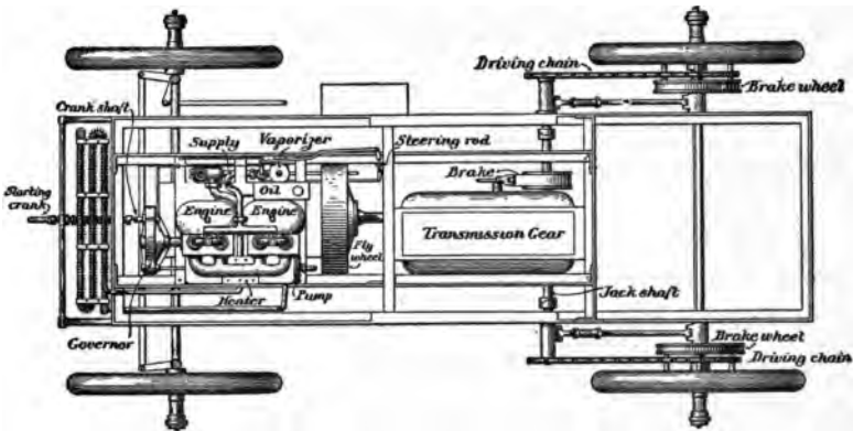
FIGS. 19, 20.—Part Sectional Elevation and Plan of the Riker-Locomobile Chassis, showing arrangement of jack-shaft, or countershaft, and double chain drive.
